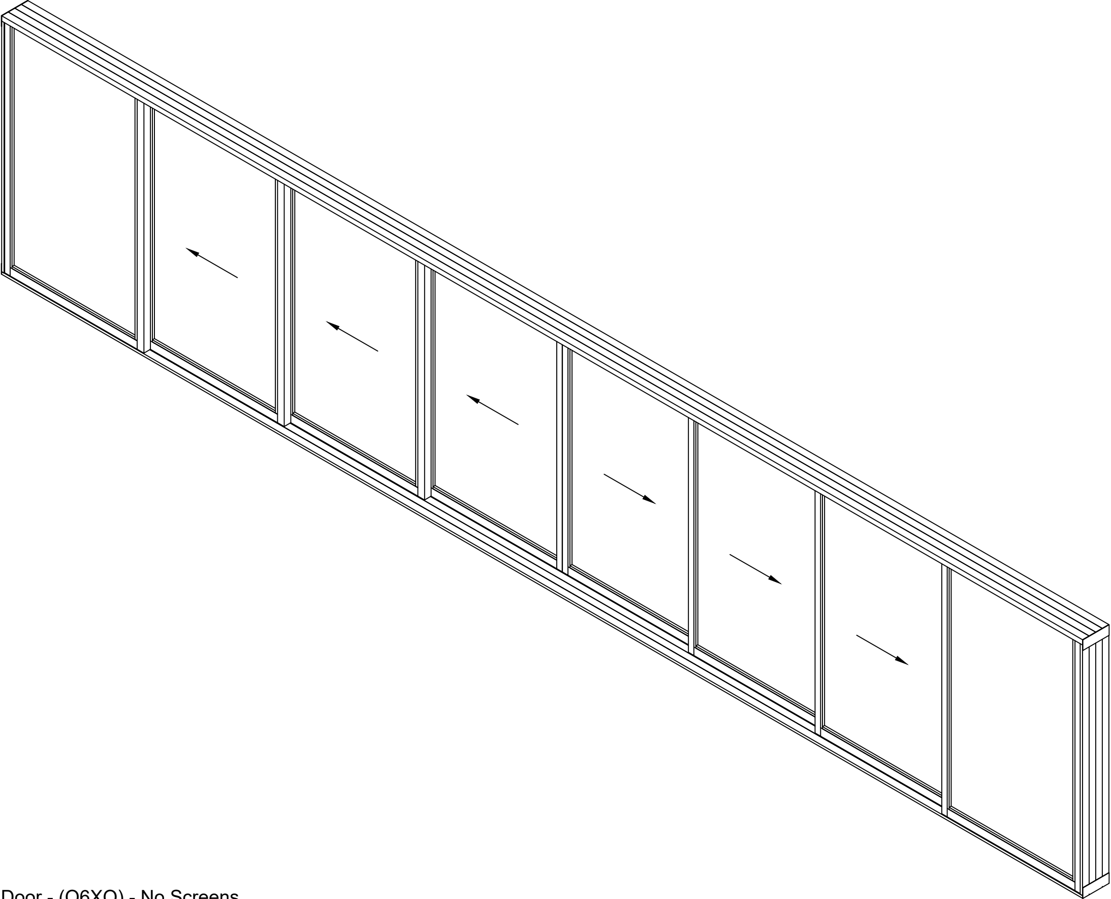
Series 8600 Multi-slide Stacking Door - (O6XO) - No Screens
