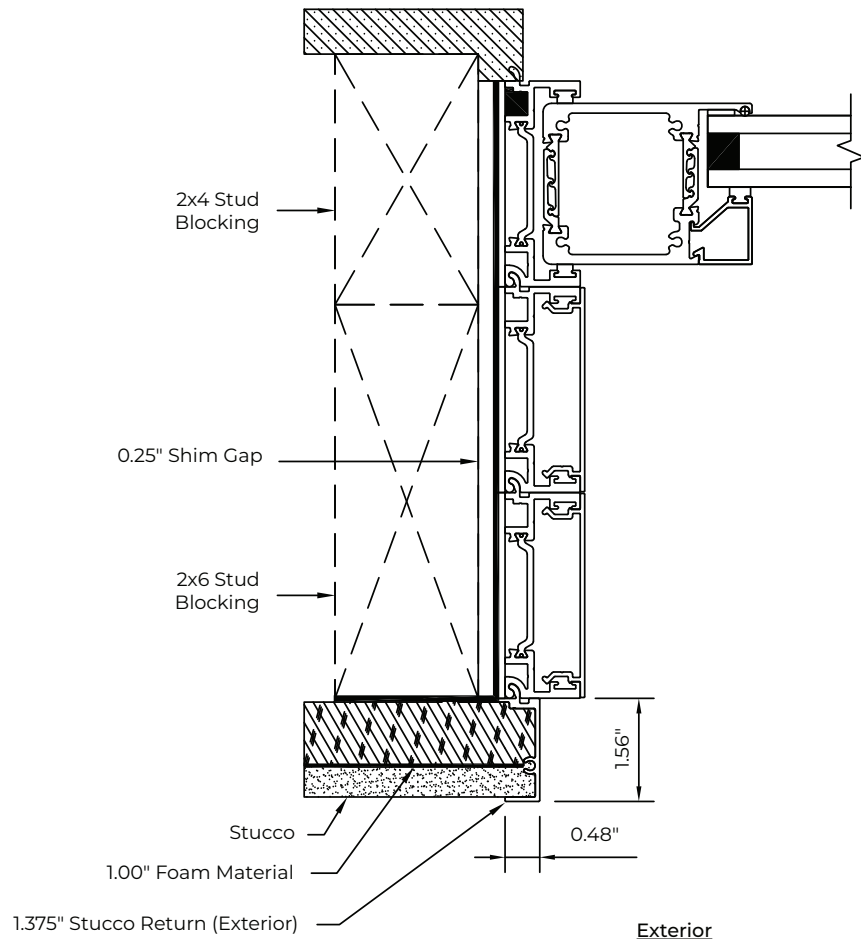
1.375" Stucco Return Wall Construction Profile At Stud Multi-Slide Door Jamb Application
