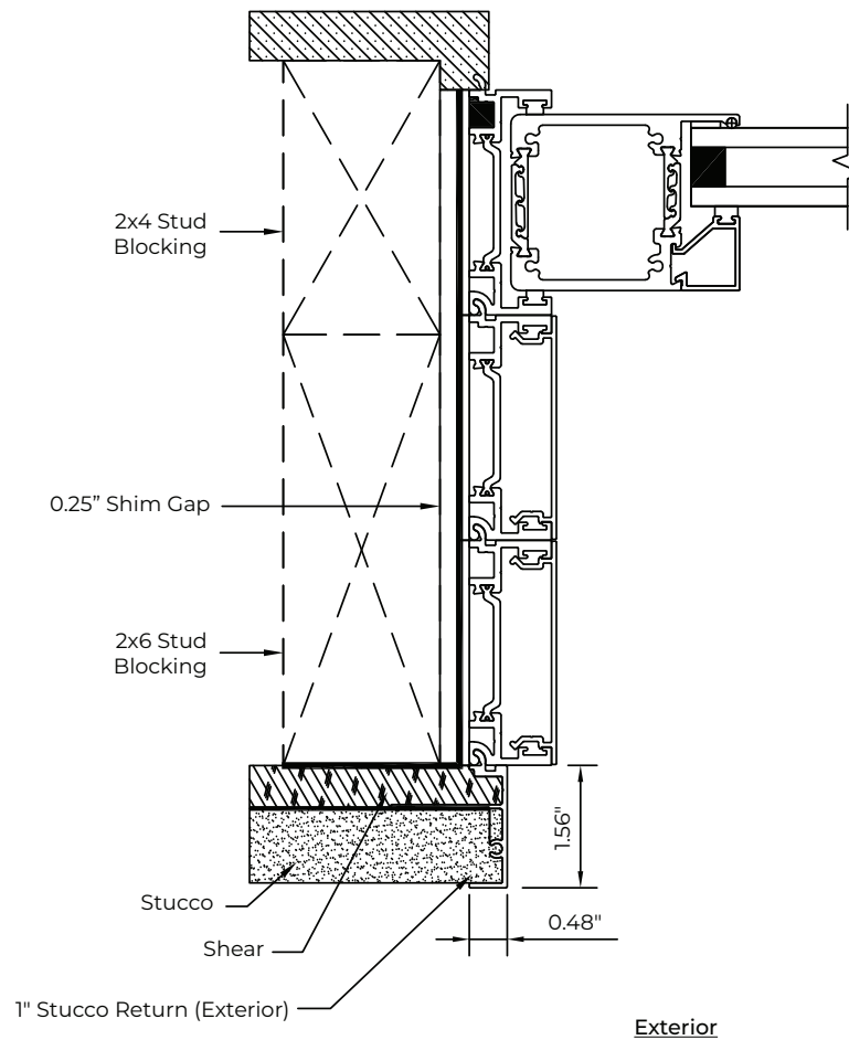
1" Stucco Return Wall Construction Profile At Stud Multi-Slide Door Jamb Application
