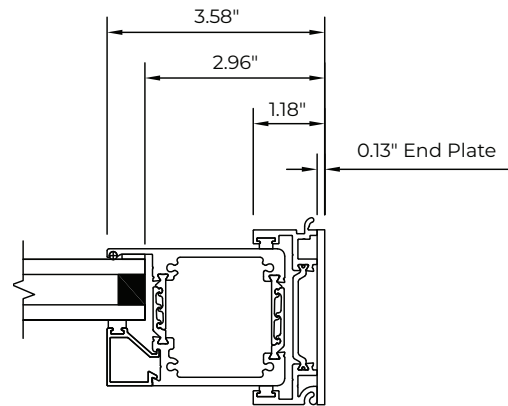
Right Jamb Condition
