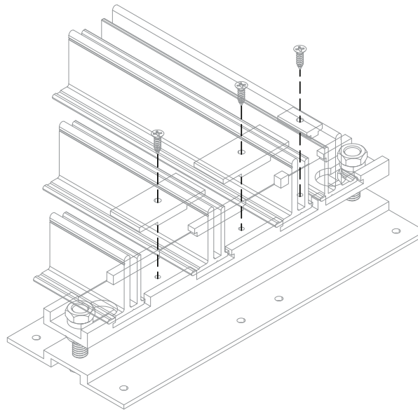
Threshold Condition At Track Clamps
