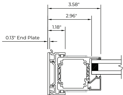
Left Jamb Condition
