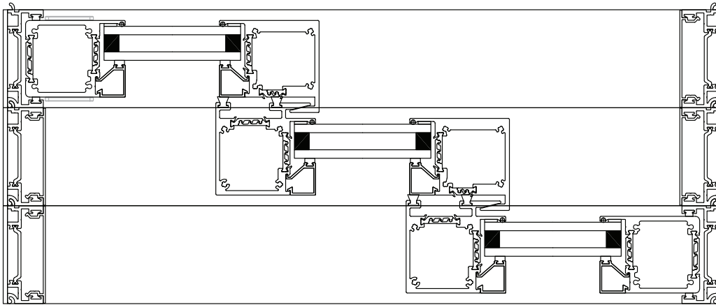
Horizontal Section Of 3-Panel Stacking Door Or 2XO
